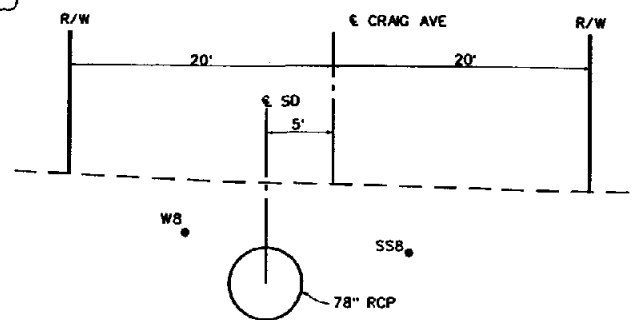
TYPICAL SECTION
