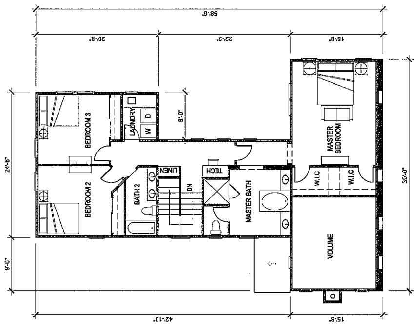
2ND FLOOR AREA = 1389 SF
