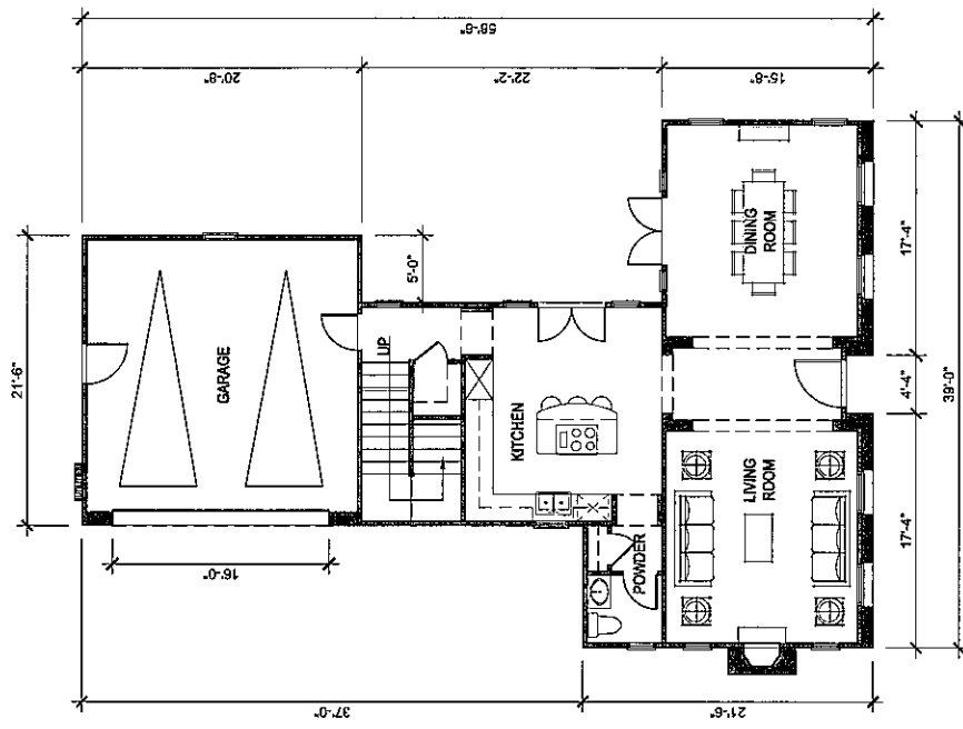
1ST FLOOR AREA = 995 SF
