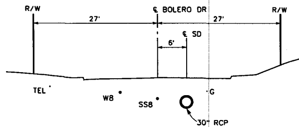
TYPICAL SECTION
