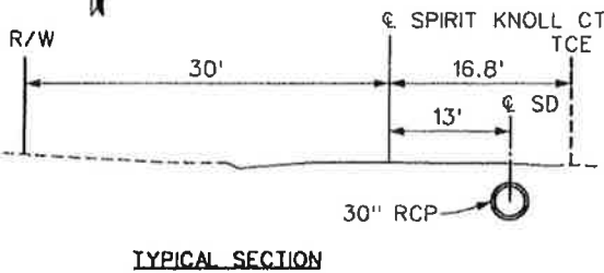
TYPICAL SECTION
