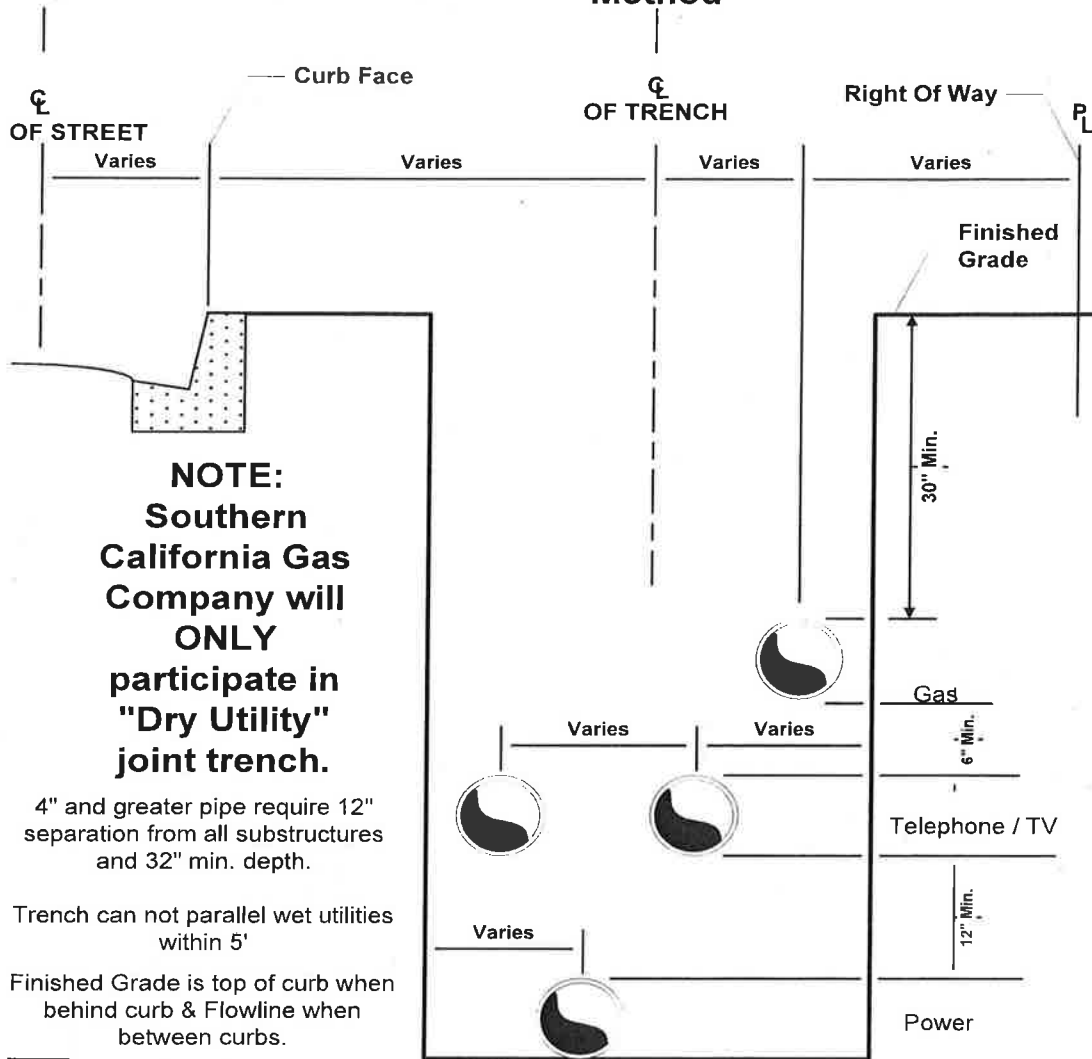
CROSS SECTION OF JOINT TRENCH NO SCALE
