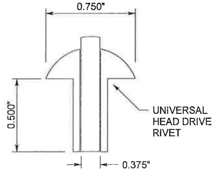
RIVET DETAIL
