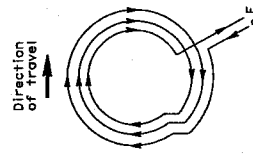
SAWCUT DETAIL TYPE E LOOP DETECTOR CONFIGURATION WINDING DETAIL
