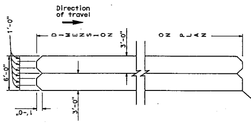
SAWCUT DETAIL TYPE C LOOP DETECTOR CONFIGURATION WINDING DETAIL
