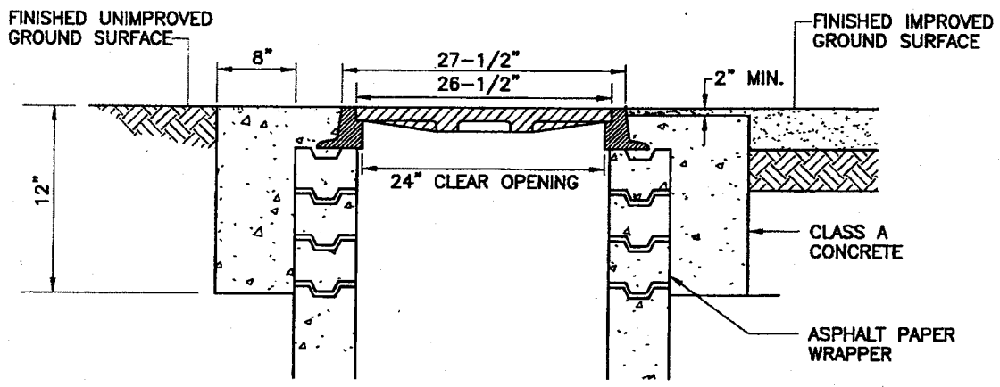
TYPICAL INSTALLATION SECTION
