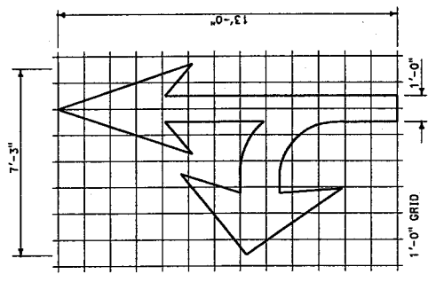
TYPE VII (L) ARROW A=27 sq ft (FOR TYPE III (R) ARROW, USE MIRROR IMAGE)
