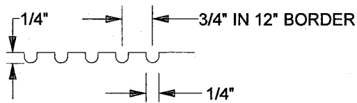
GROOVING DETAIL
