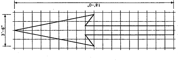
TYPE I 18'-0" ARROW A=25 sq ft
