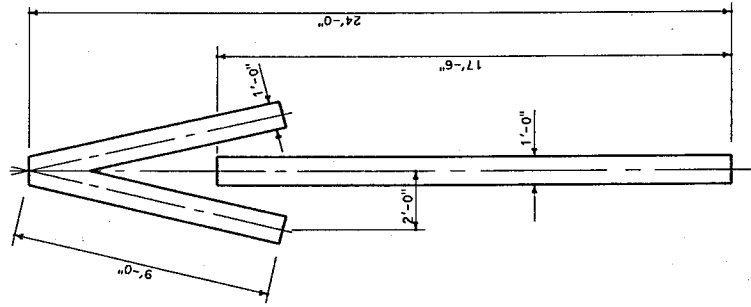
TYPE V ARROW A=33 sq ft
