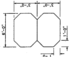
SAWCUT DETAIL TYPE Q LOOP DETECTOR CONFIGURATION WINDING DETAIL
