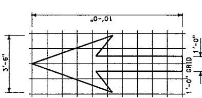
TYPE I 10'-0" ARROW A=14 sq ft
