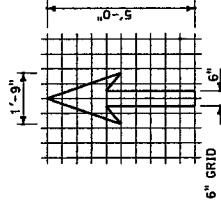
TYPE VI ARROW A=42 sq ft RIGHT LANE DROP ARROW (FOR LEFT LANE, USE MIRROR IMAGE)
