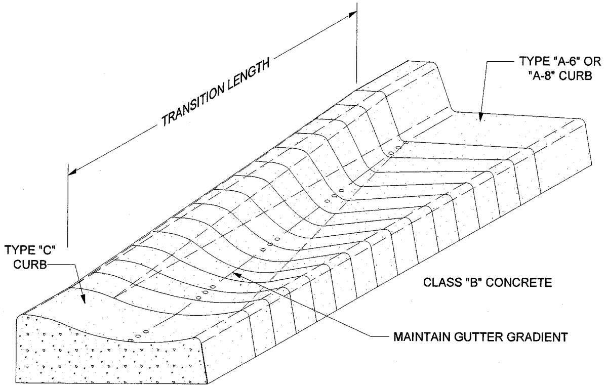
ISOMETRIC VIEW
