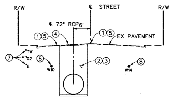
TYPICAL SECTION AT STA 25+00
