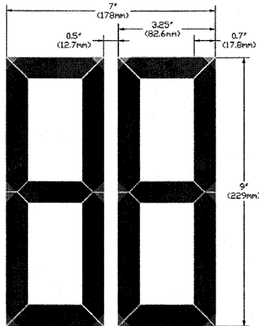
Figure 2: Countdown Display
