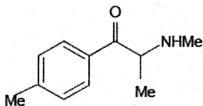
MEPHEDRONE
