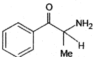
CATHINONE
