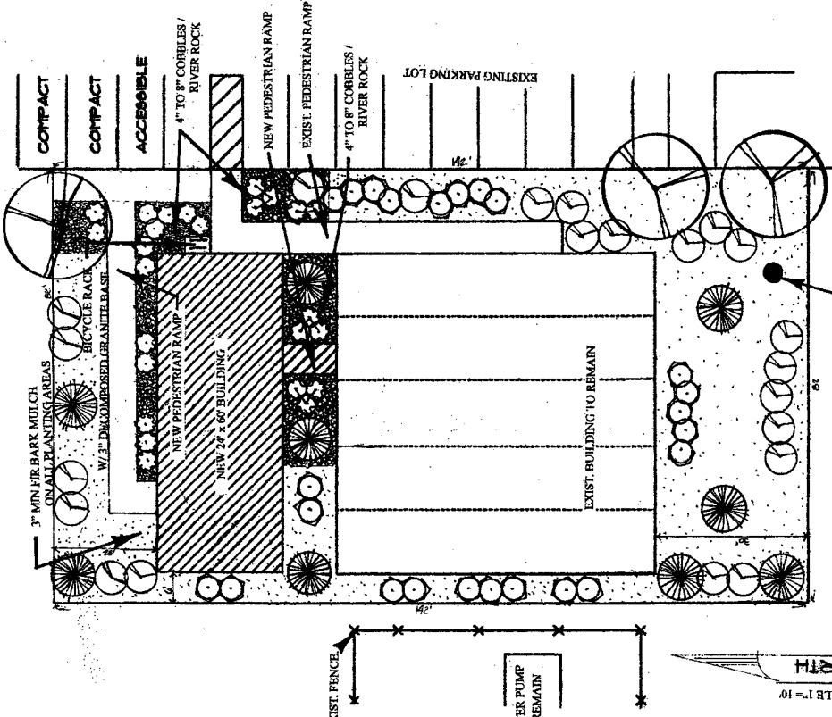
LANDSCAPE PLAN
