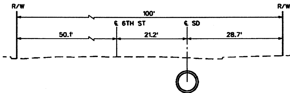
Typical Reinforced Concrete Pipe Section
