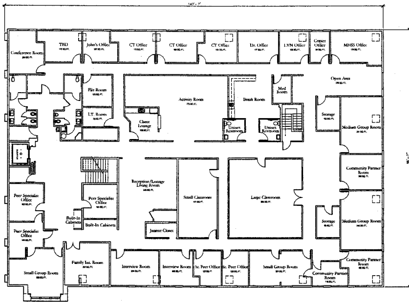
Proposed "Upper Level" Floor Plan
