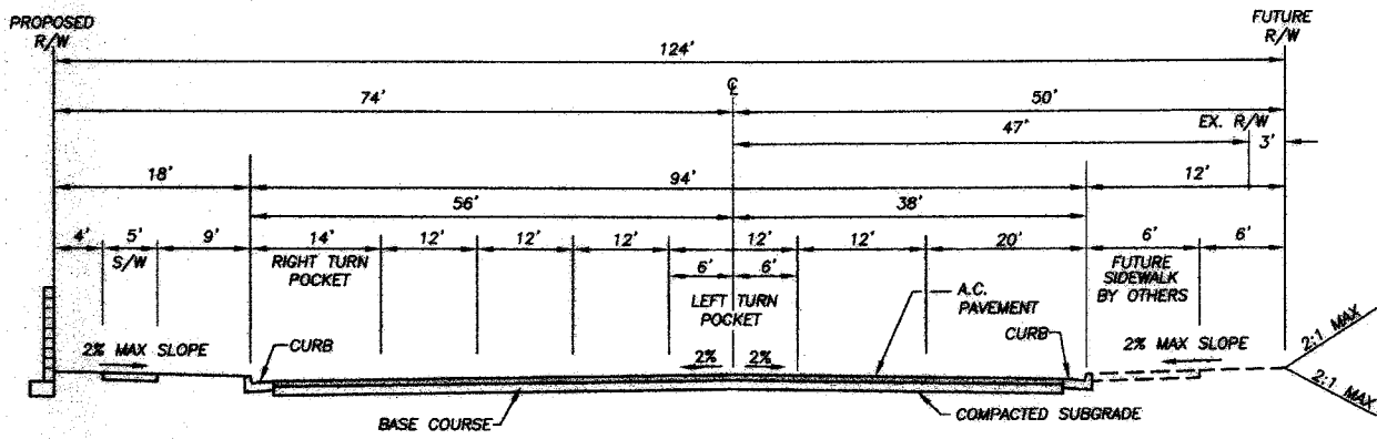
TYPICAL SECTION SECONDARY HIGHWAY STD. No. 94 MODIFIED PER THIRD SUPERVISORIAL DISTRICT STANDRDS RICE ROAD (STA. 13+85.28 TO 14+00.63) NTS (T.I.=7.0, R=6, A.C.=0.33', A.B=1.43')
