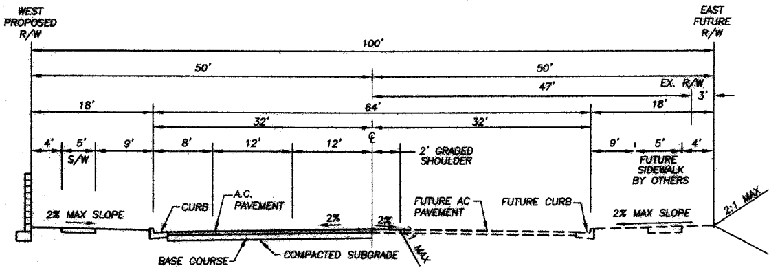
TYPICAL SECTION SECONDARY HIGHWAY STD. No. 94 MODIFIED PER THIRD SUPERVISORIAL DISTRICT STANDRDS RICE ROAD (STA. 17+53.83 TO 24+53.53) NTS (T.I.=7.0, R=6, A.C.=0.33', A.B=1.43')
