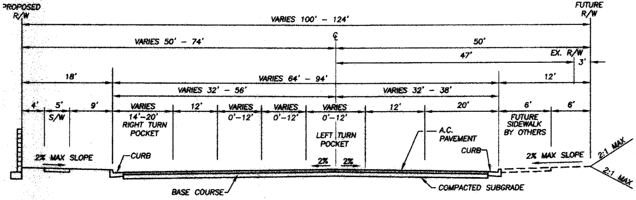
TYPICAL SECTION SECONDARY HIGHWAY STD. No. 94 MODIFIED PER THIRD SUPERVISORIAL DISTRICT STANDRDS RICE ROAD (STA. 14+00.63 TO 17+53.83) NTS (T.I.=7.0, R=6, A.C.=0.33', A.B=1.43')
