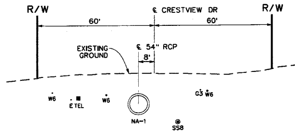
SECTION AT STA 4+50
