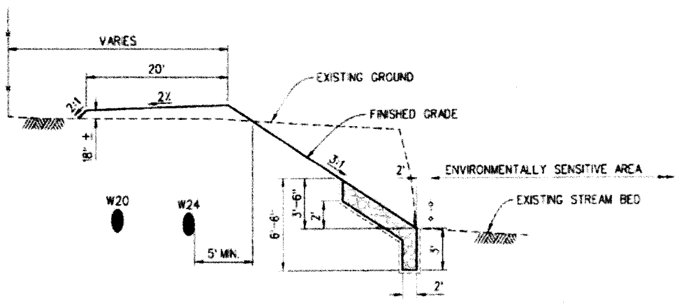
ROCK RIPRAP REVETMENT TYPICAL SECTION C 1
