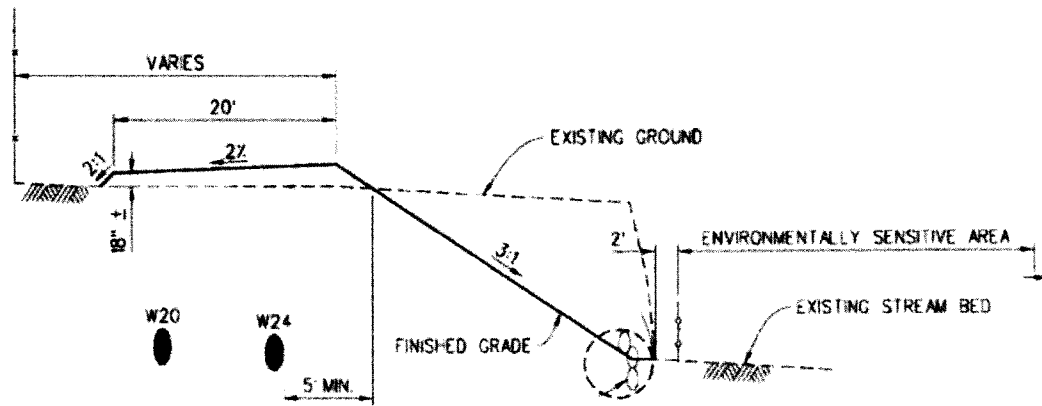
BANK TYPICAL SECTION A 2
