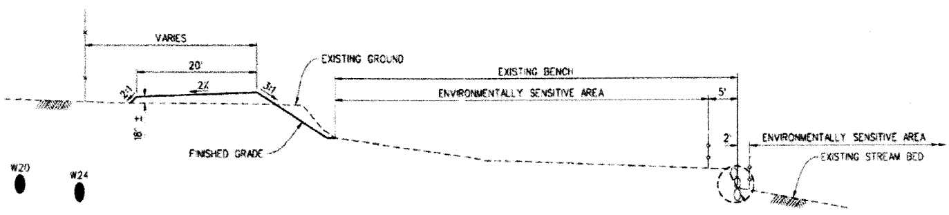
BANK (WITH BENCH) TYPICAL SECTION B 2
