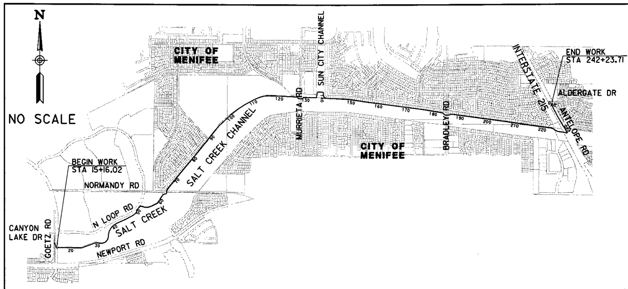
VICINITY MAP
