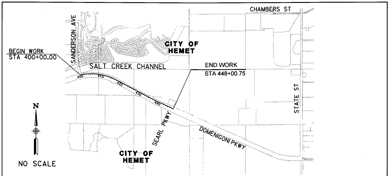
VICINITY MAP
