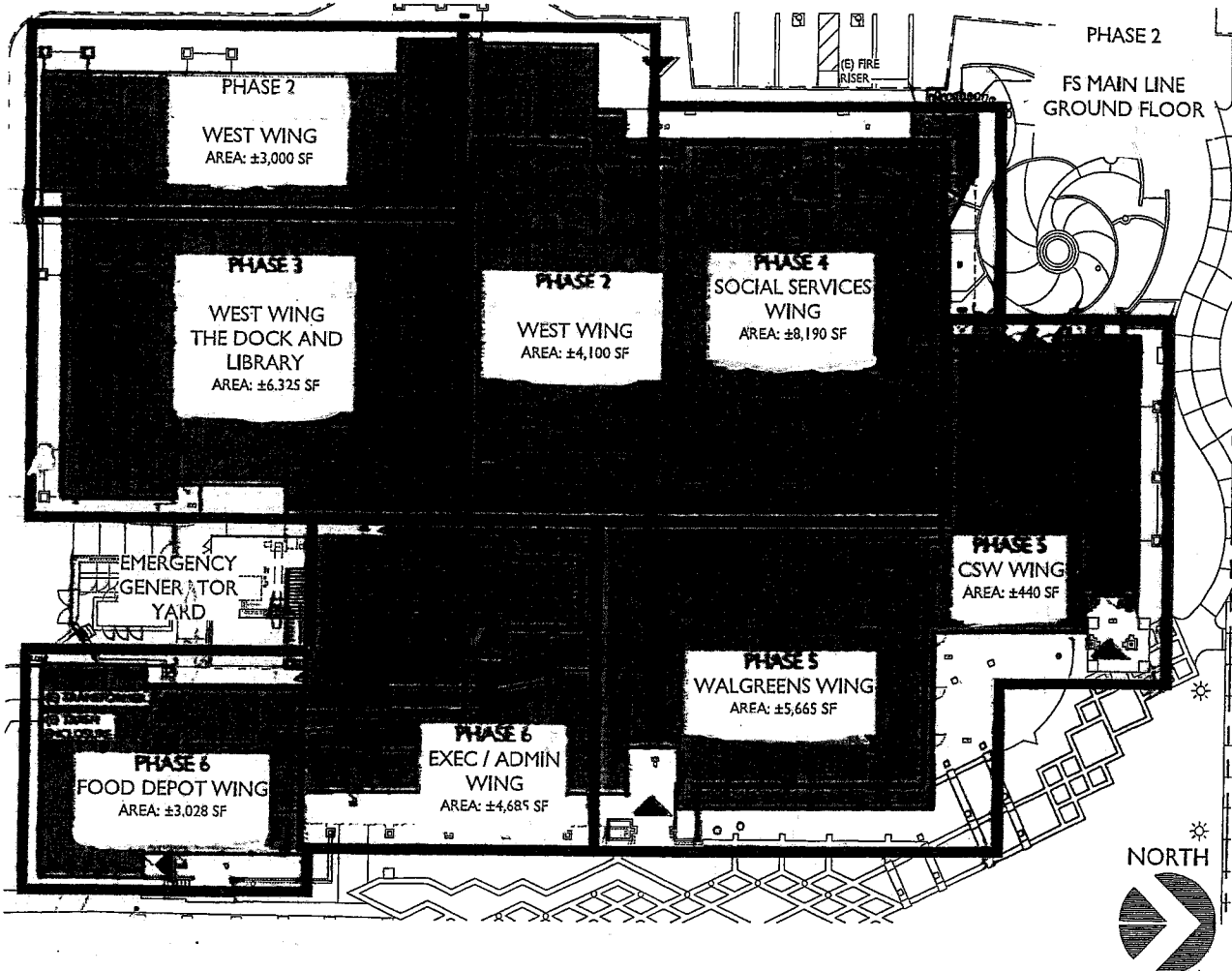
DAP - SITE & PHASING PLAN
