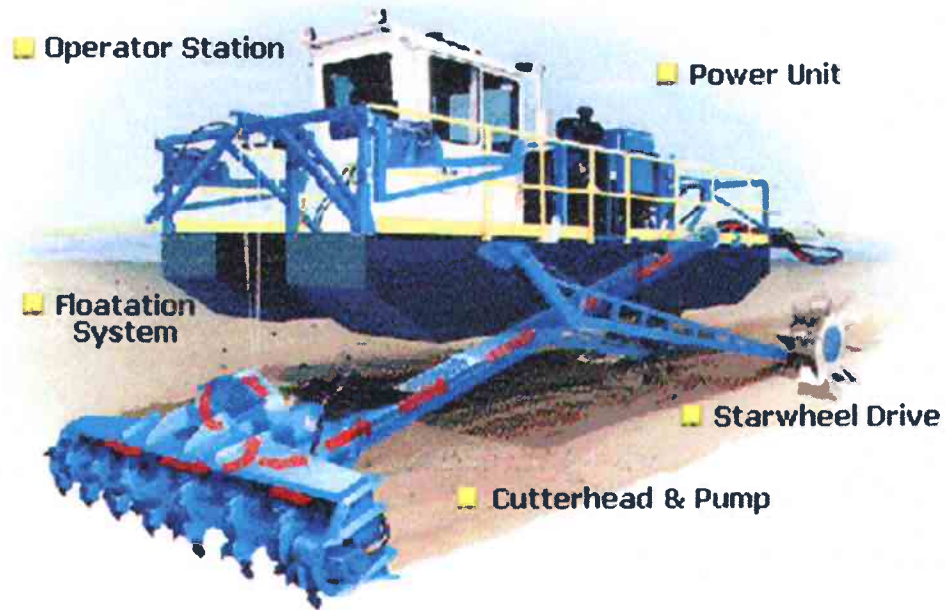
Figure 4 Hydraulic Dredge Illustration 3
