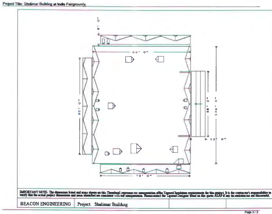
Tapered Roof Diagram
