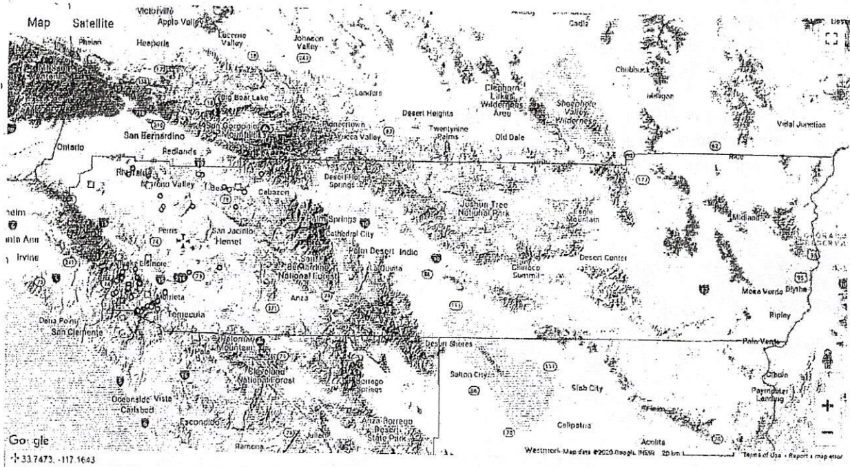
Known Centaurea solstitialis distribution in Riverside County according to Calflora on 1/27/2020
