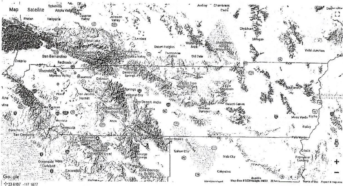
Known Dittrichia graveolens distribution in Riverside County according to Calflora on 1/27/2020. There are more unmapped populations within Temescal Valley (parallels the 15 freeway north of the mapped points).
