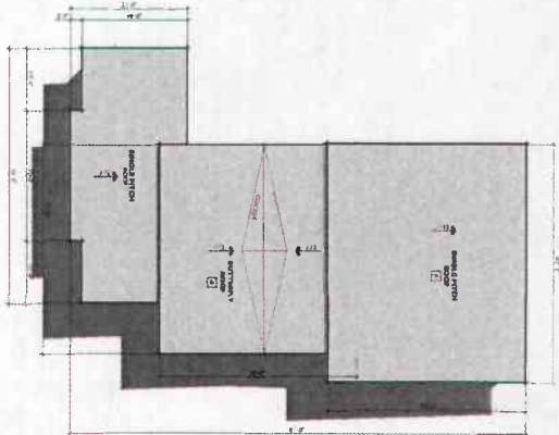
ROOF PLAN SCALE 3/32" = 1'-0"
