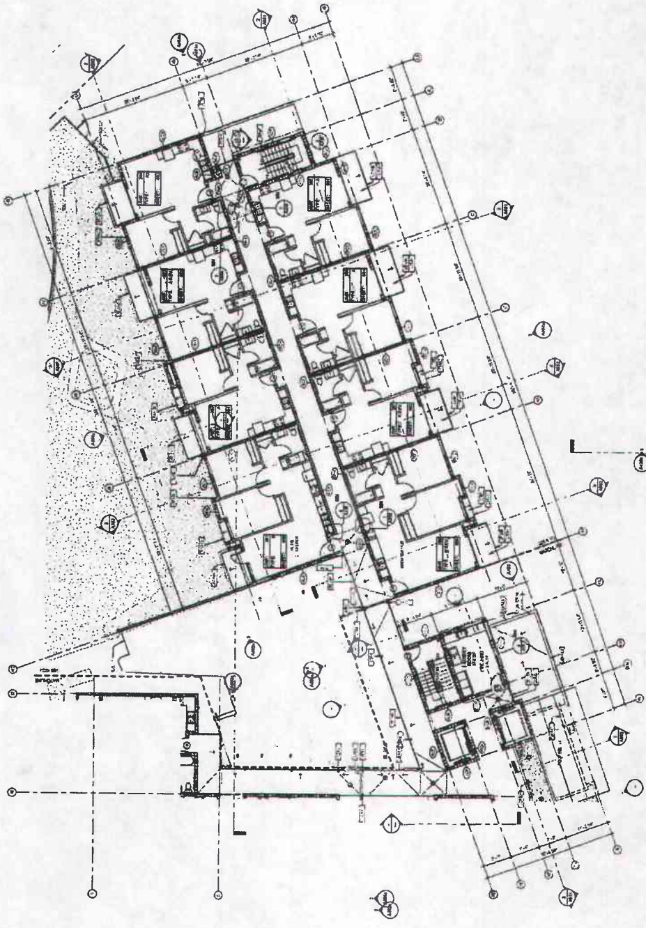
1 SECOND FLOOR PART B - 18" x 1'-0"
