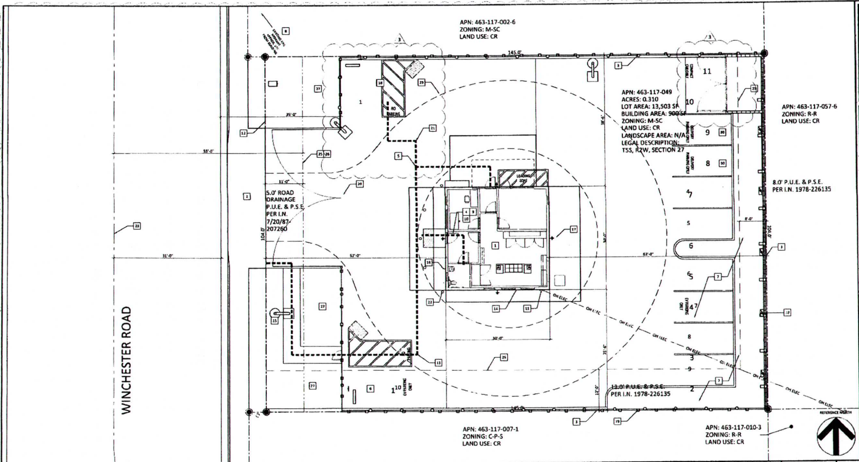
SITE PLAN SCALE 1" = 40'-0" 1
