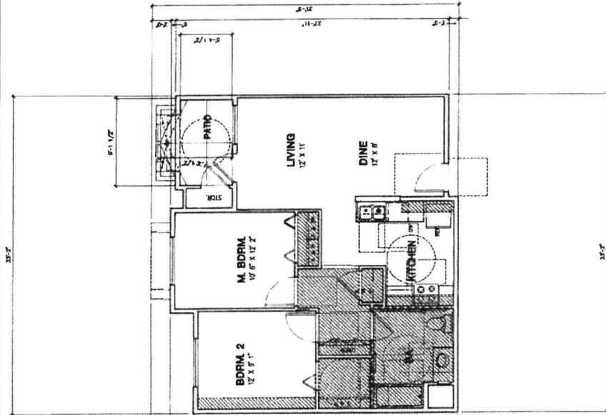
UNIT B1.1 2 BEDROOM - 1 BATH ADAPTABLE & ACCESSIBLE UNIT AT FIRST FLOOR LEVEL
