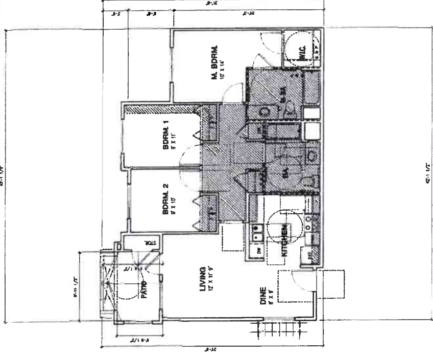
UNIT C11 3 BEDROOM - 2 BATH ADAPTABLE & ACCESSIBLE UNIT AT FIRST FLOOR LEVEL
