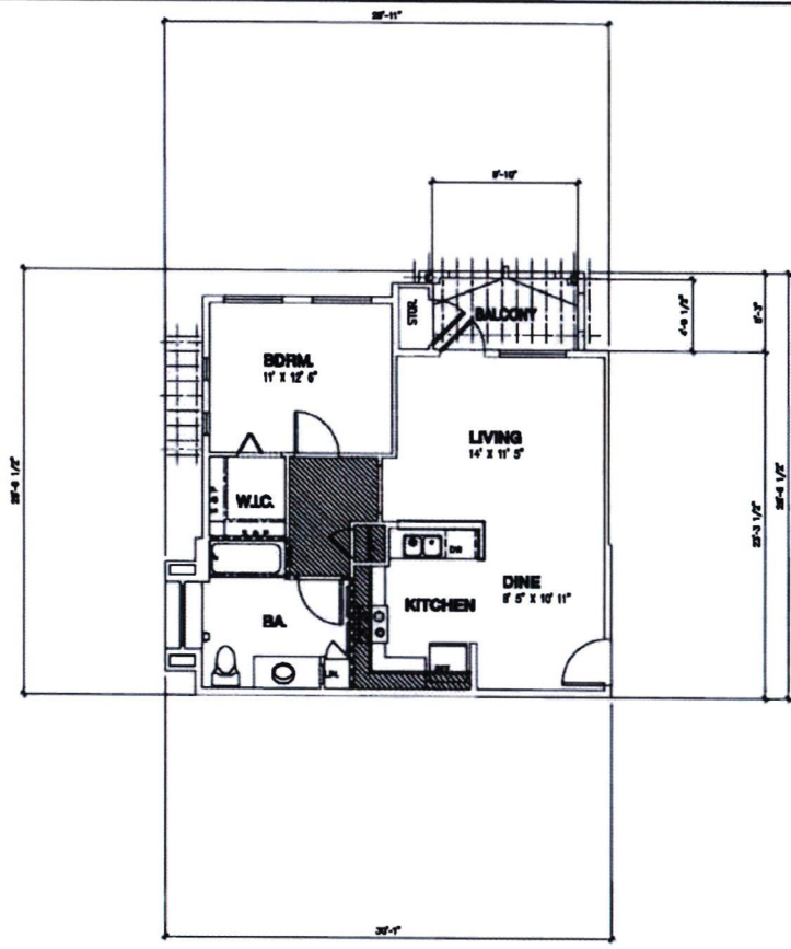
UNIT A2 UPPER LEVEL UNIT 1 BEDROOM - 1 BATH SCALE: 1/4" = 1'-0"
