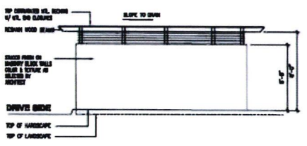
LEFT SIDE ELEVATION
