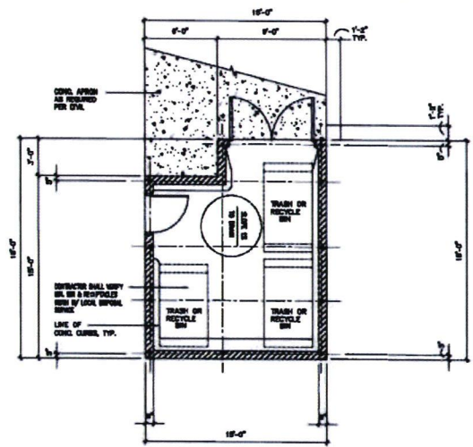
FLOOR PLAN 252 SQ. FT. TRASH OR RECYCLE ENCLOSURE SCALE: 1/4" = 1'-0" REFER TO ARCHITECTURAL SITE PLAN (AS.1) FOR TRASH & RECYCLE ENCLOSURE LOCATIONS
