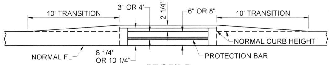
PROFILE
