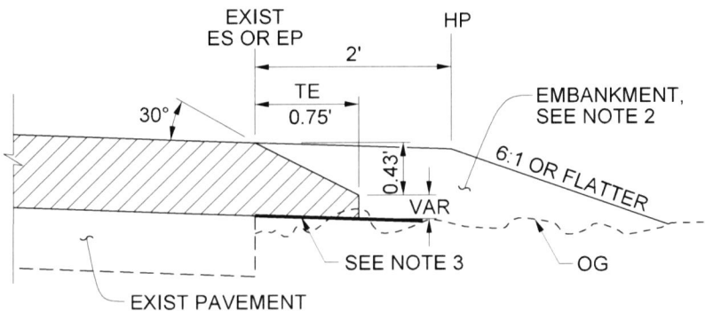
DETAIL "A" FOR HMA OVERLAY THICKNESS MORE THAN 0.43'.
