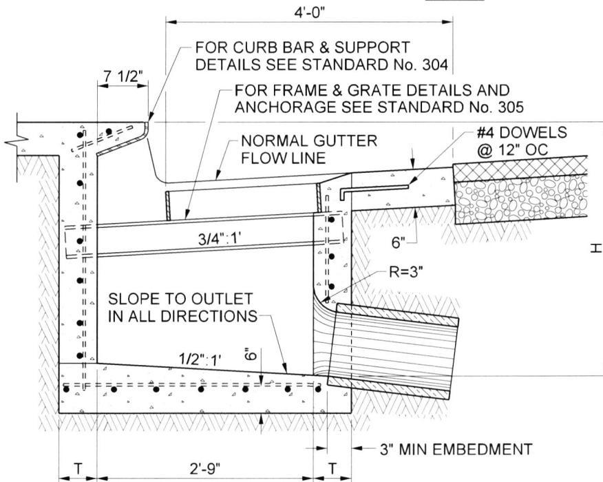
SECTION "A-A"
