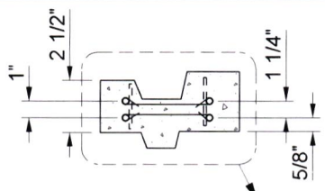
24" x 2 1/2" GRADE RING
