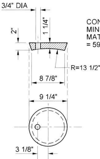
CAST IRON COVER
