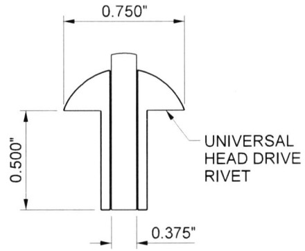
RIVET DETAIL
