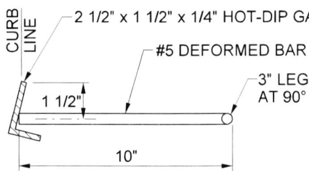
ANCHOR DETAIL
