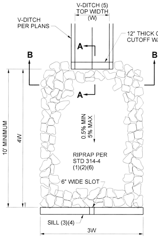
PLAN
