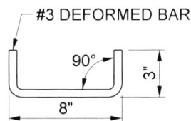
DOWEL DETAIL
