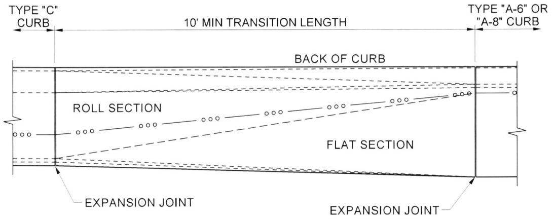
PLAN VIEW
