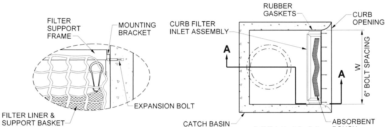
DETAIL "B-B" TOP VIEW
