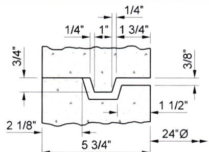
JOINT DETAIL "A"
