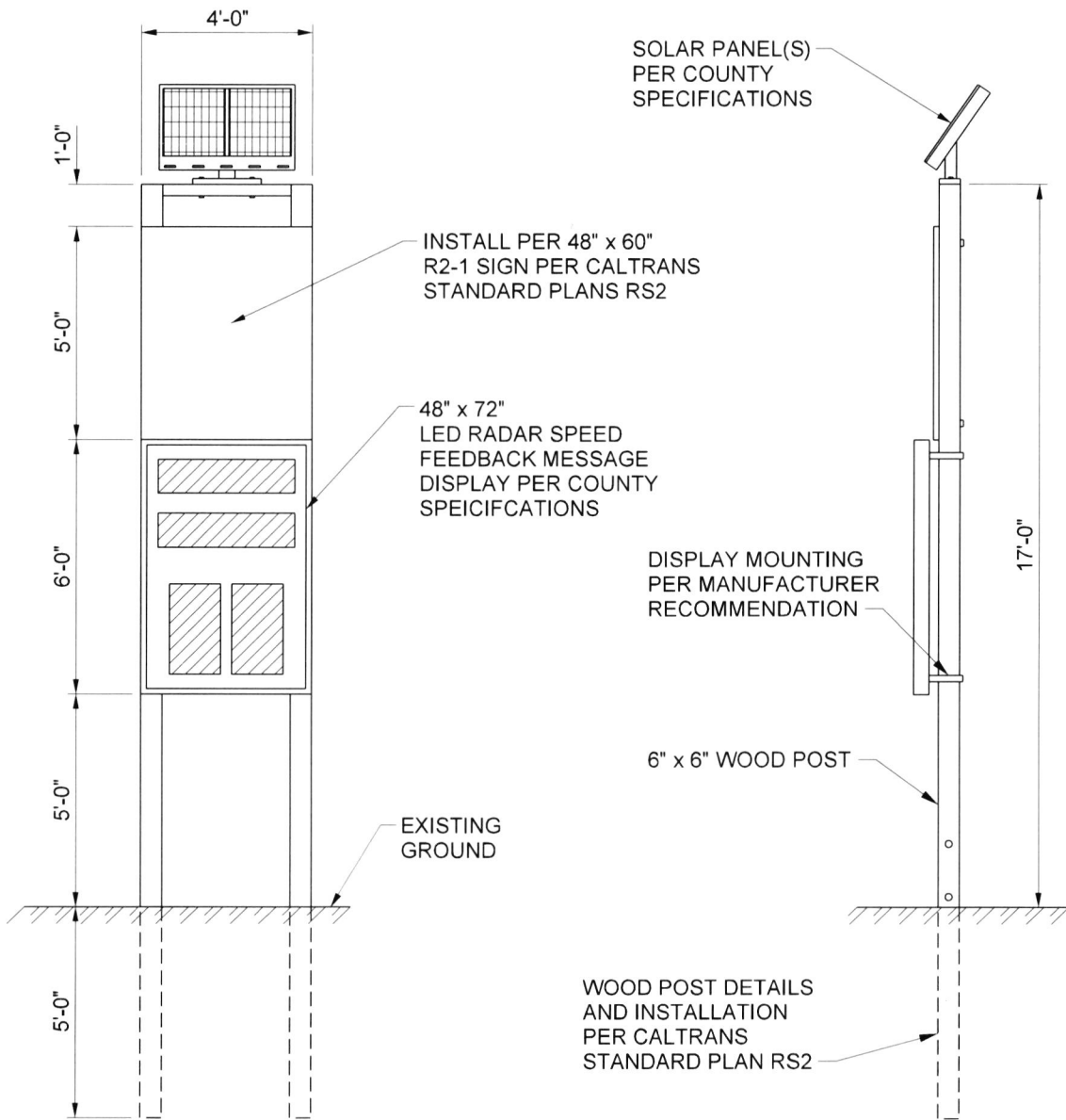
FRONT VIEW
