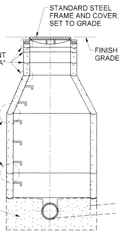
TYPICAL SECTION
