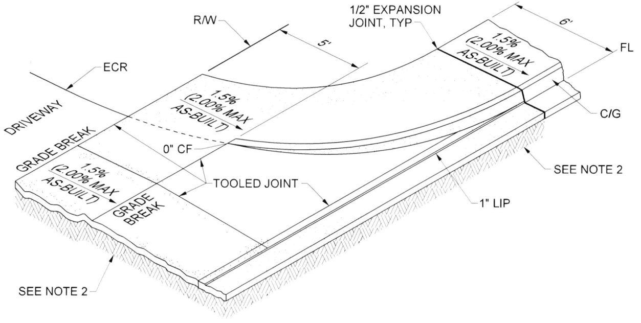
ISOMETRIC VIEW
