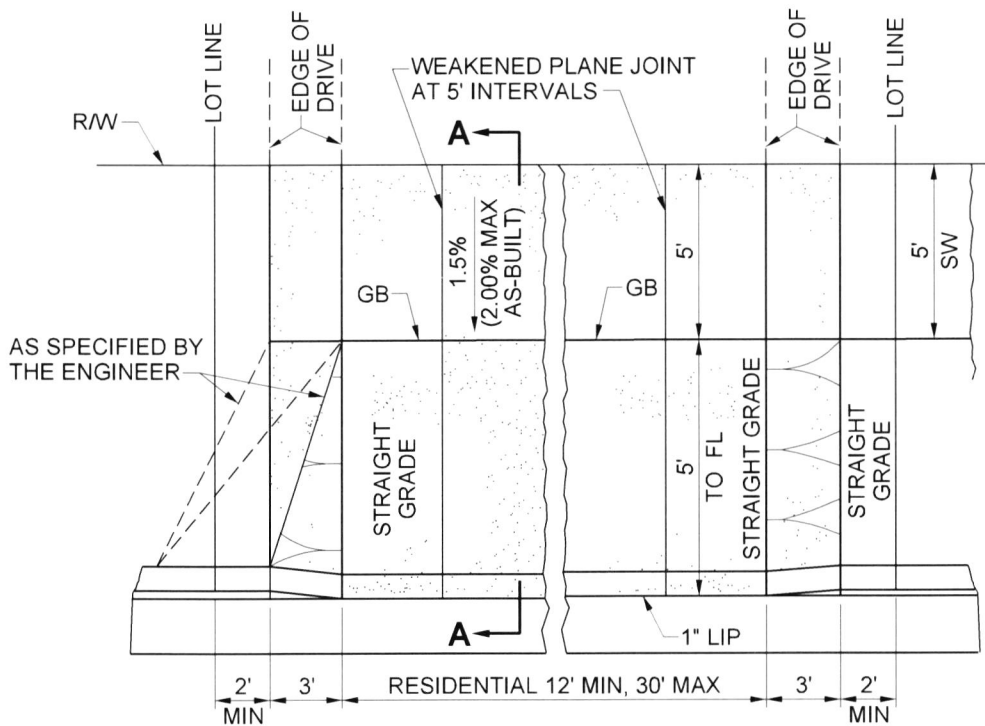
WHEN NO SIDEWALK EXISTS OR IS NOT REQUIRED
