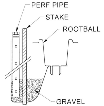
DRAIN PIPE DETAIL 4" SCH 40 PERF PIPE 1 PER TREE
