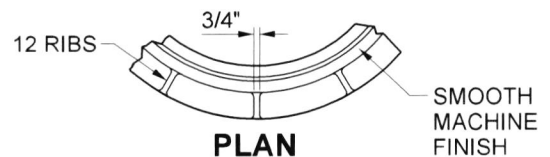
PLAN PORTION OF FRAME
