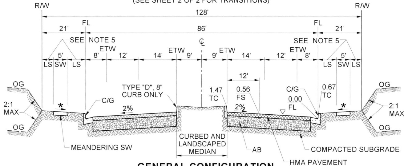
GENERAL CONFIGURATION
