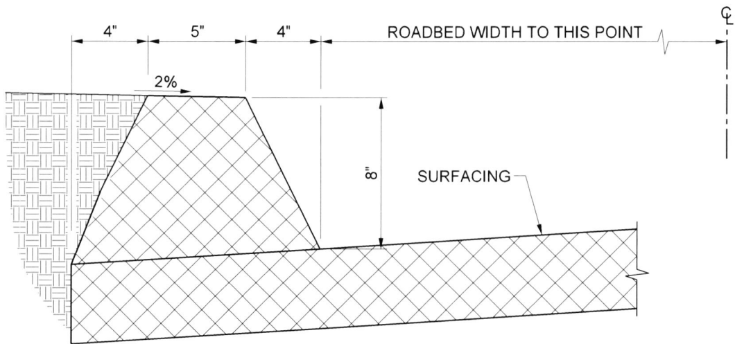
8" HMA DIKE
