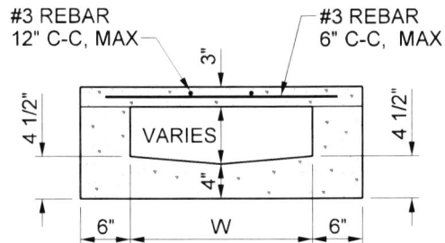
SECTION "X-X"
