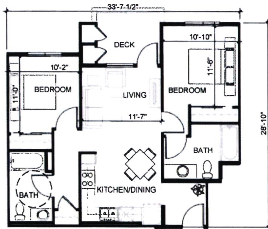
Unit Type 2-1 2 Bedrooms/ 2 Bathrooms Net Area: 772 SQ. FT. Gross Area: 820 SQ. FT.
