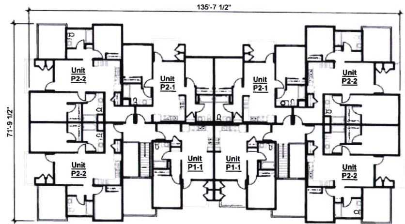
2nd Floor
