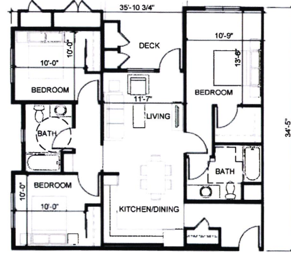
Unit Type 3-1 3 Bedrooms/ 2 Bathrooms Net Area: 1012 SQ. FT. Gross Area: 1082 SQ. FT.
