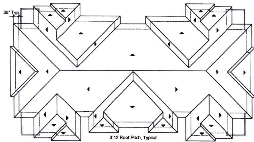
Roof Plan
