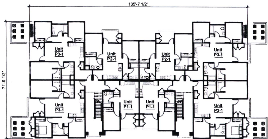
1st Floor
