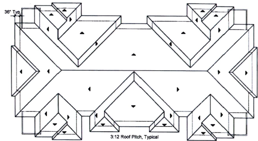
Roof Plan
