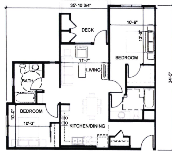
Unit Type 2-2 2 Bedrooms/ 2 Bathrooms Net Area: 882 SQ. FT. Gross Area: 944 SQ. FT.
