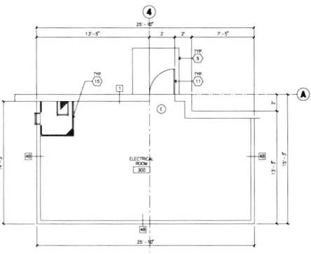
ENLARGED ELECTRICAL ROOM SCALE: 1/4" = 1'-0"
