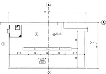
REFLECTED CEILING PLAN SCALE: 1/4" = 1'-0"
