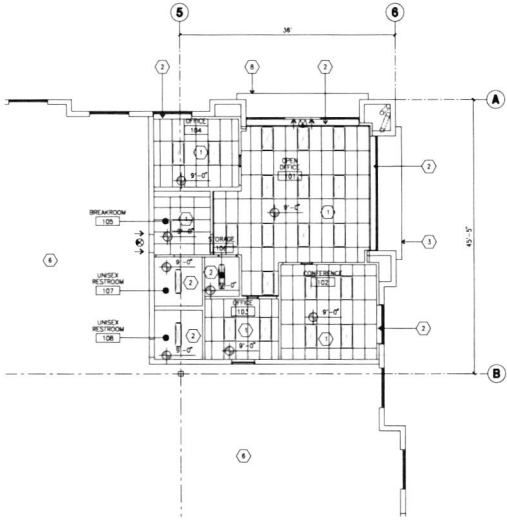
REFLECTED CEILING PLAN SCALE: 1/4" = 1'-0"
