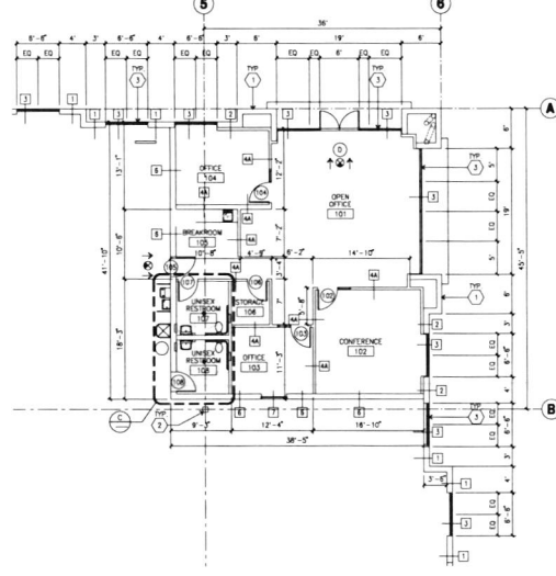
ENLARGED FLOOR PLAN SCALE: 1/4" = 1'-0"
