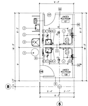
ENLARGED RESTROOM SCALE: 1/4" = 1'-0"
