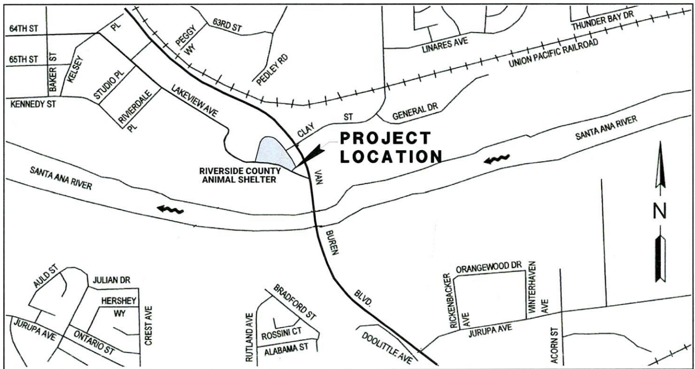
VICINITY MAP
