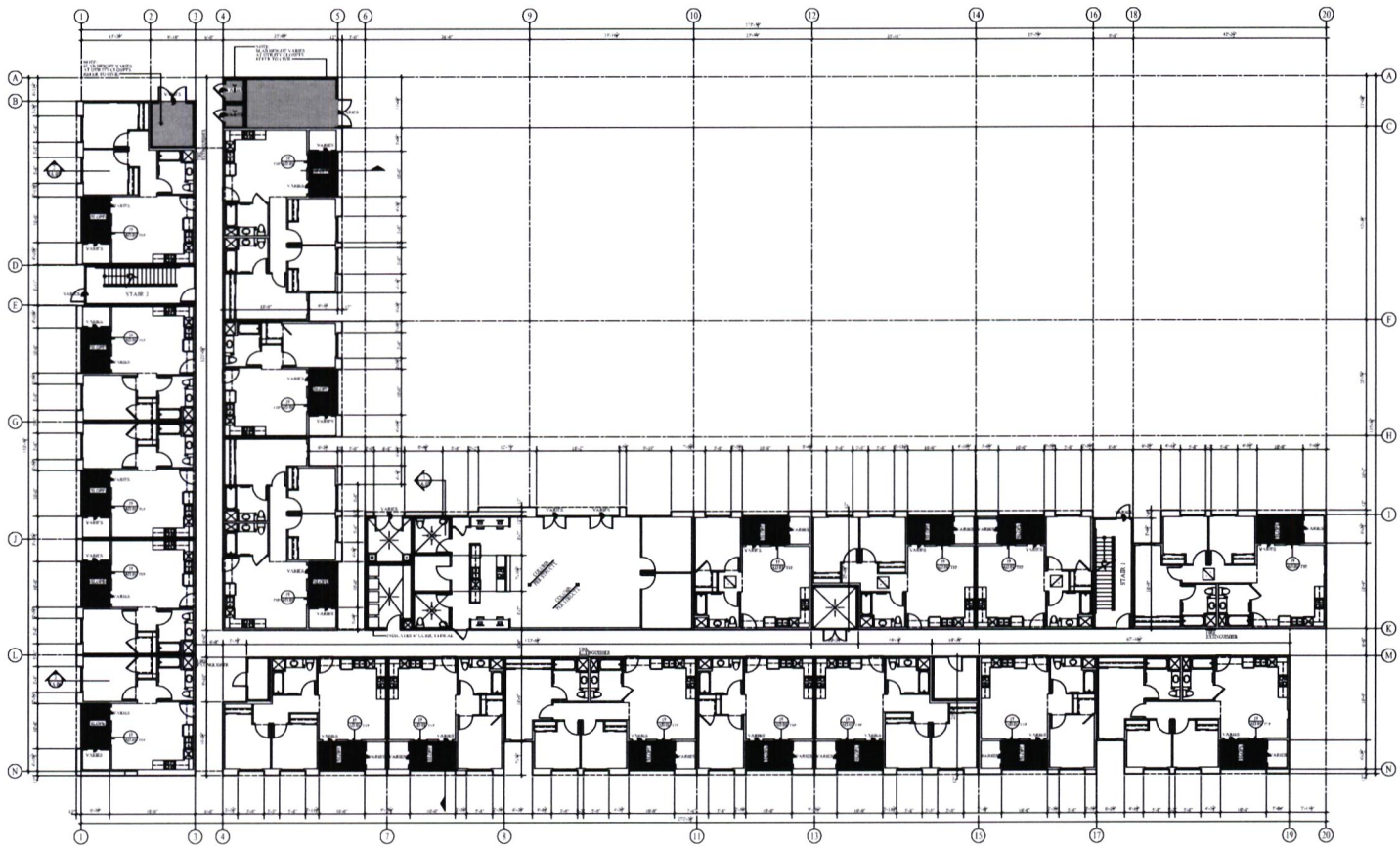
SLAB PLAN
