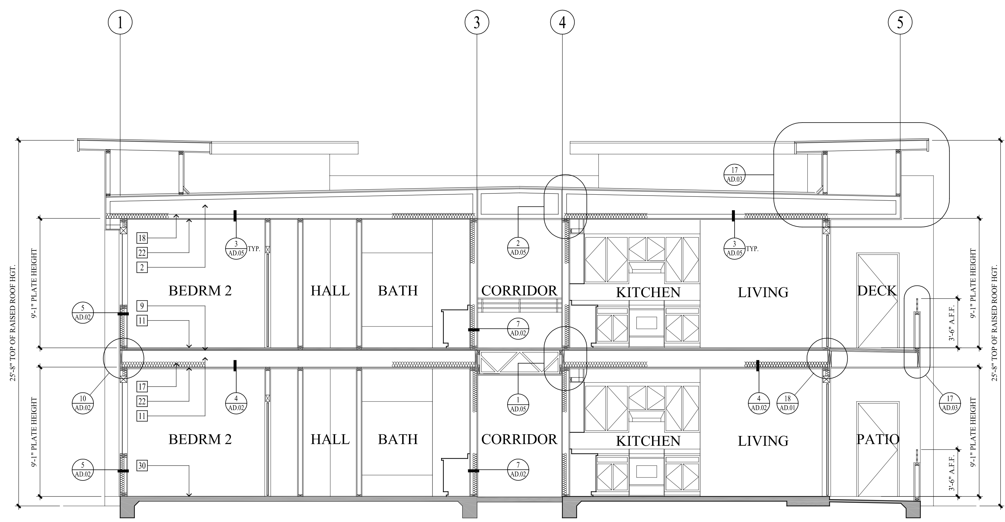
BUILDING SECTION
