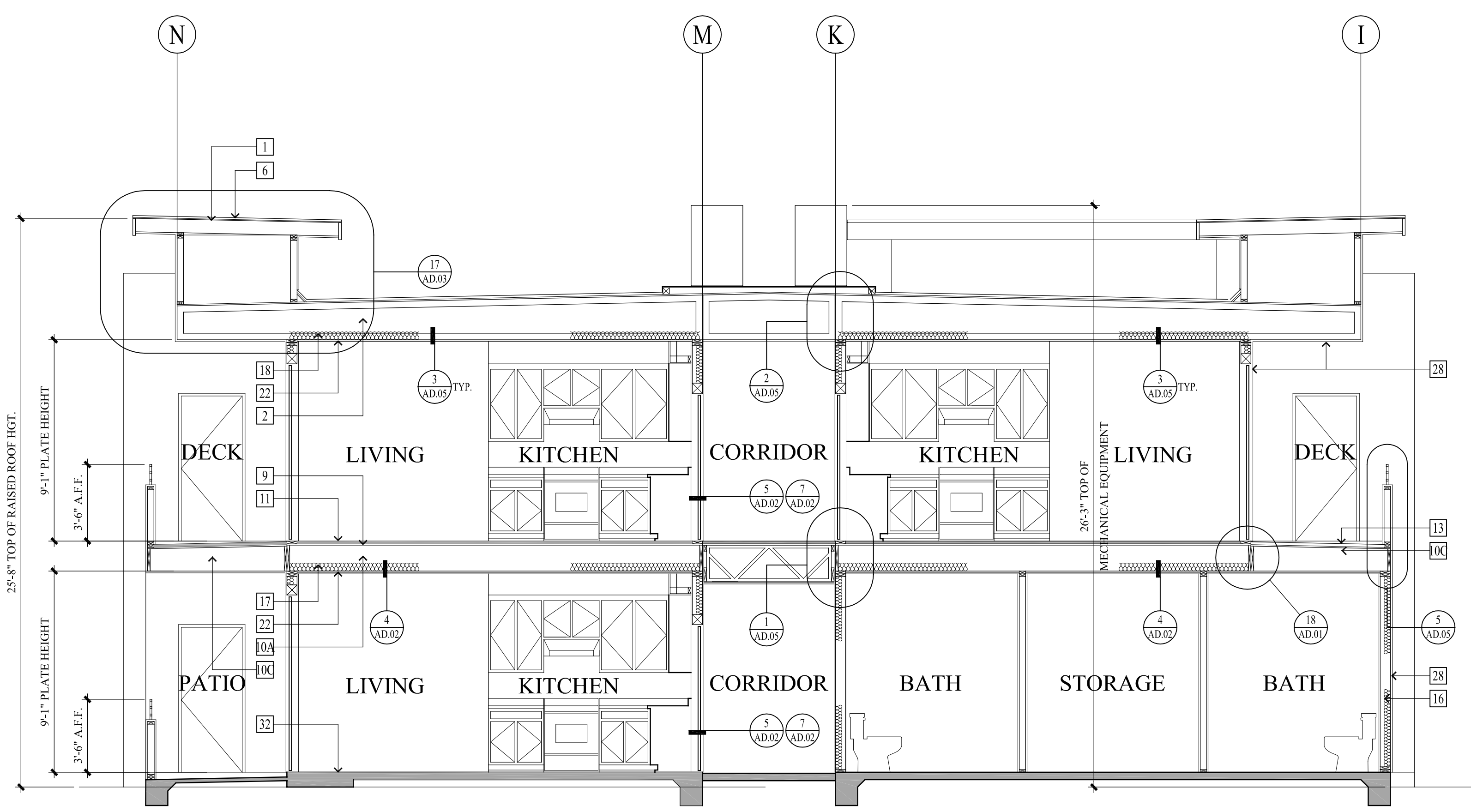
BUILDING SECTION
