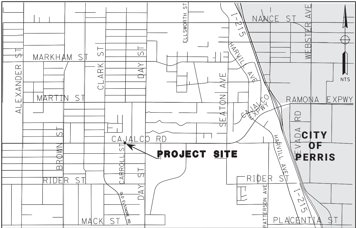
VICINITY MAP
