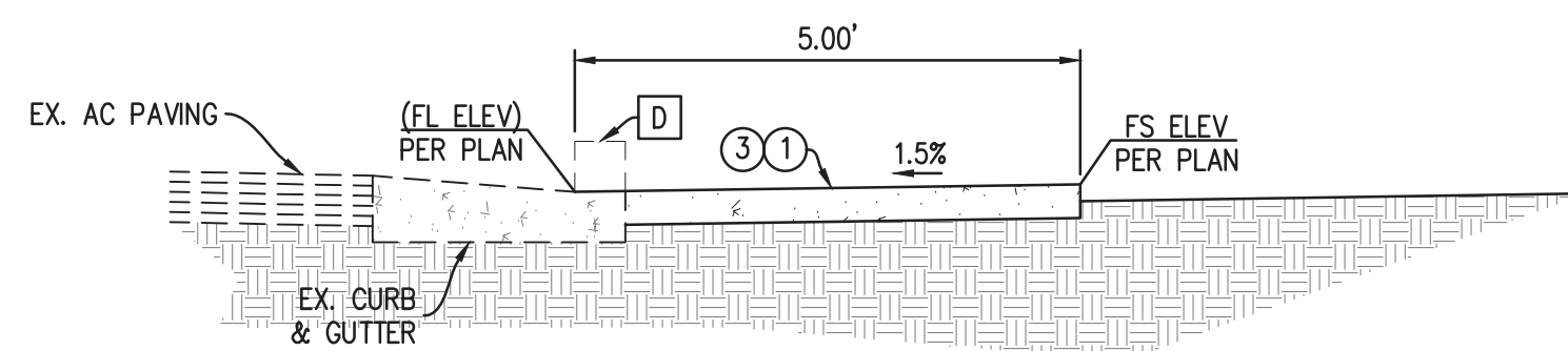
SECTION B-B
