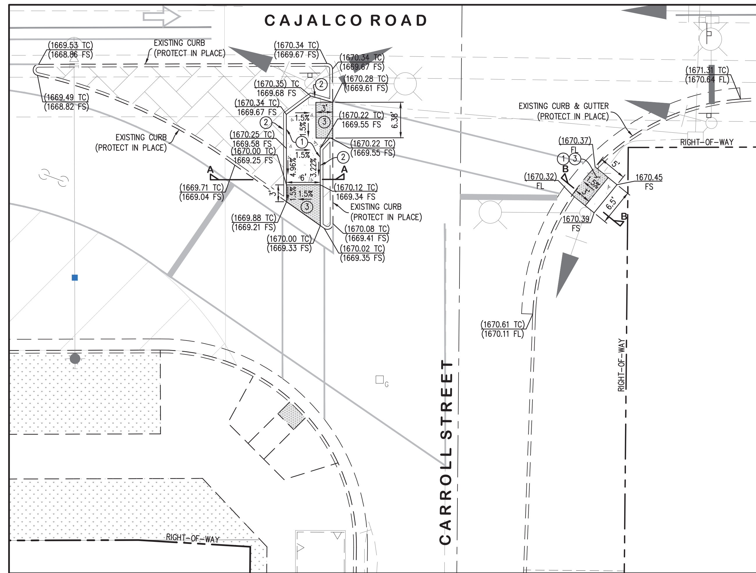
CROSSWALK PLAN
