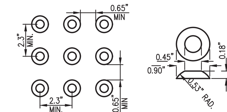
TRUNCATED DOMES DETAIL
