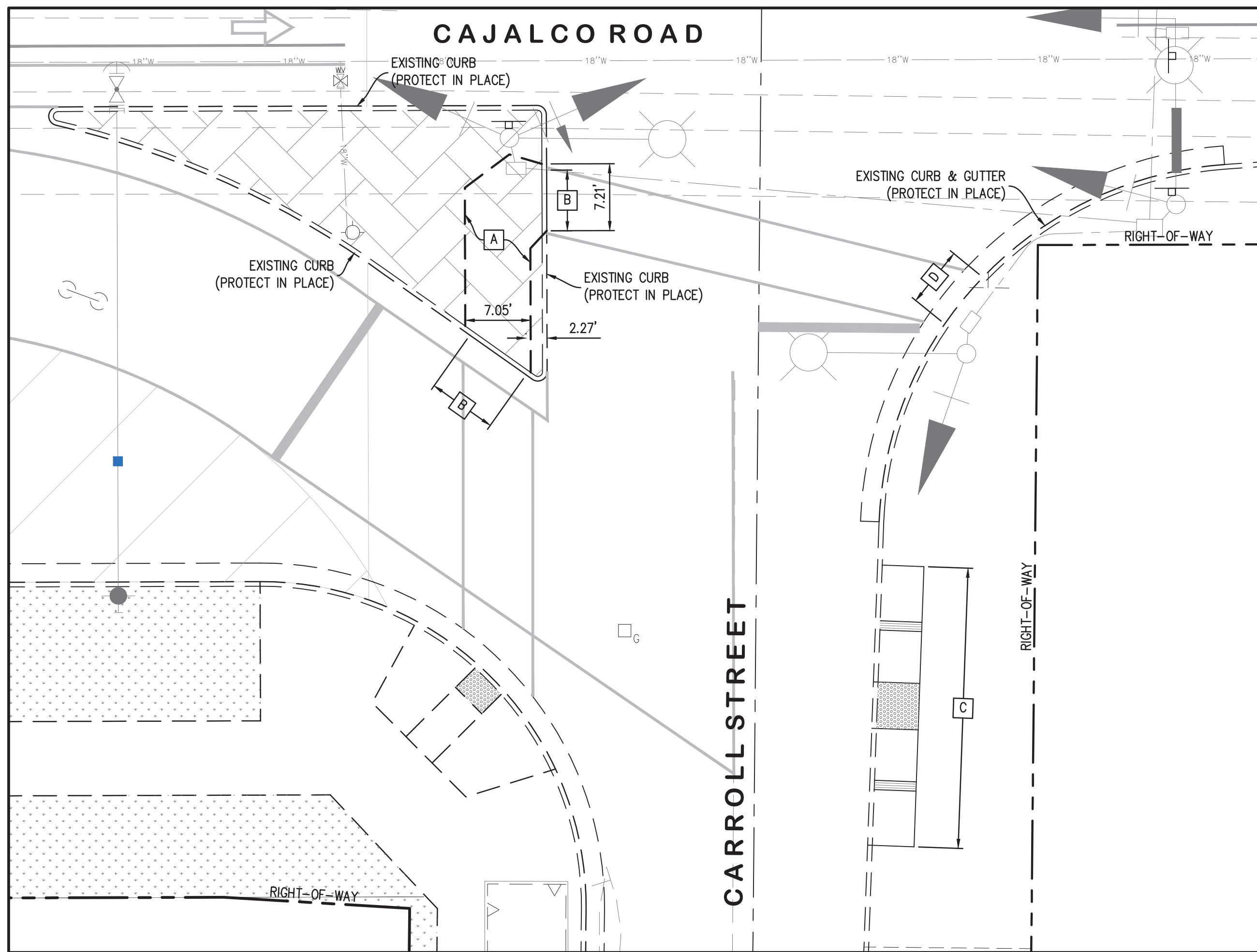
DEMOLITION PLAN
