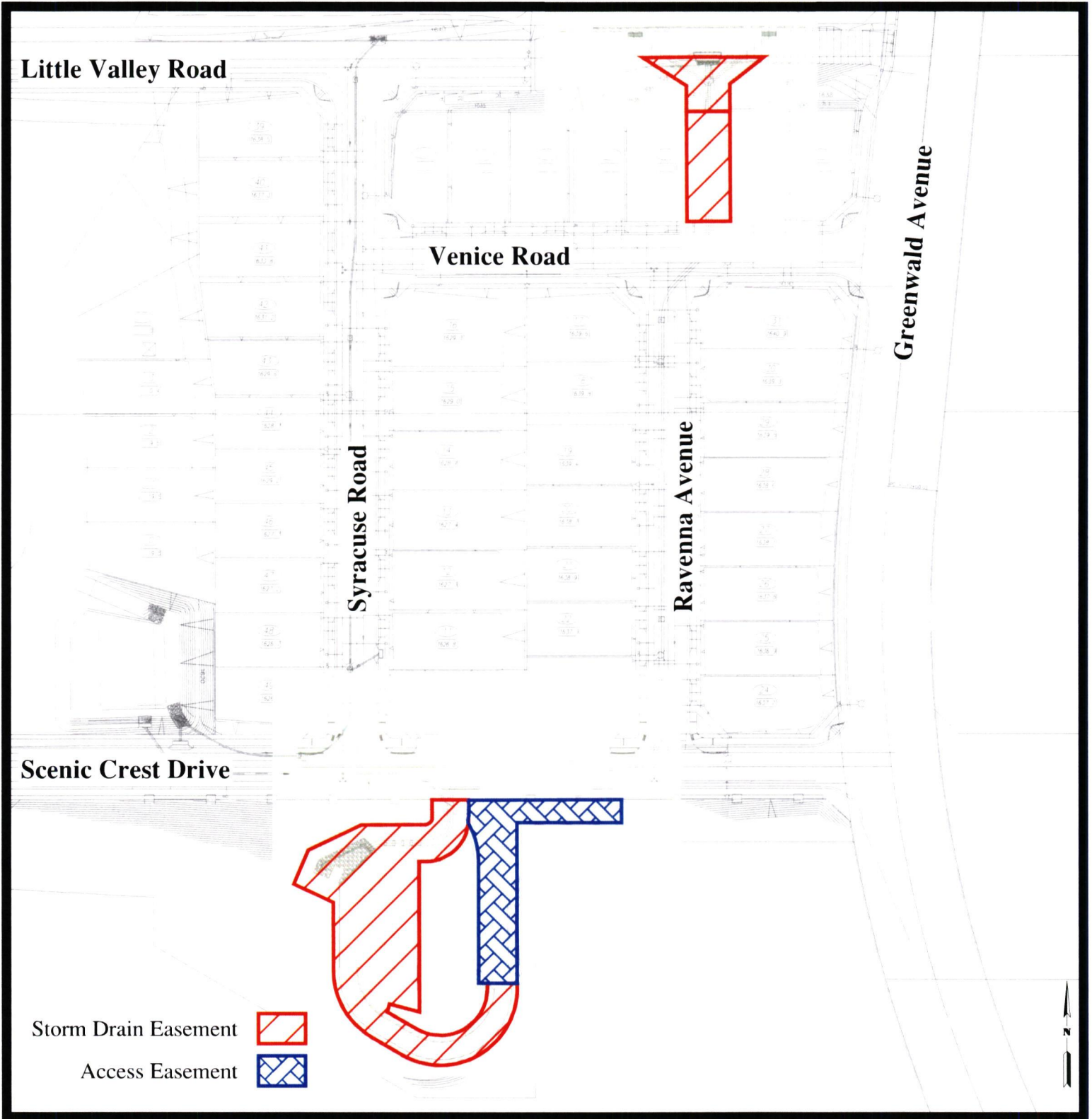
Lake Elsinore - Scenic Crest Drive Storm Drain Project No. 3-0-00055 TR 33725 (FC-85525022) Drawing No. 3-0232
